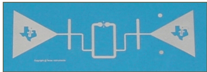
A Texas Instruments UHF RFID Tag
